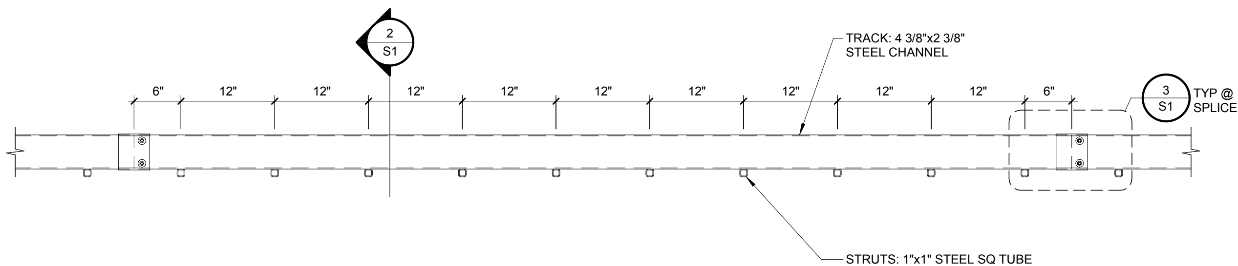
1 TRACK DETAIL S1 1" = 1'-0"
